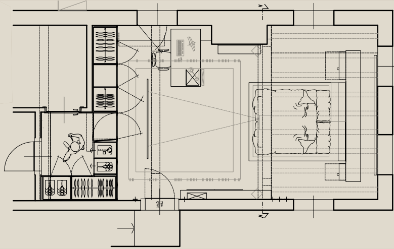
PRIMO PIANO first floor
